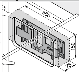
Wandmontage
